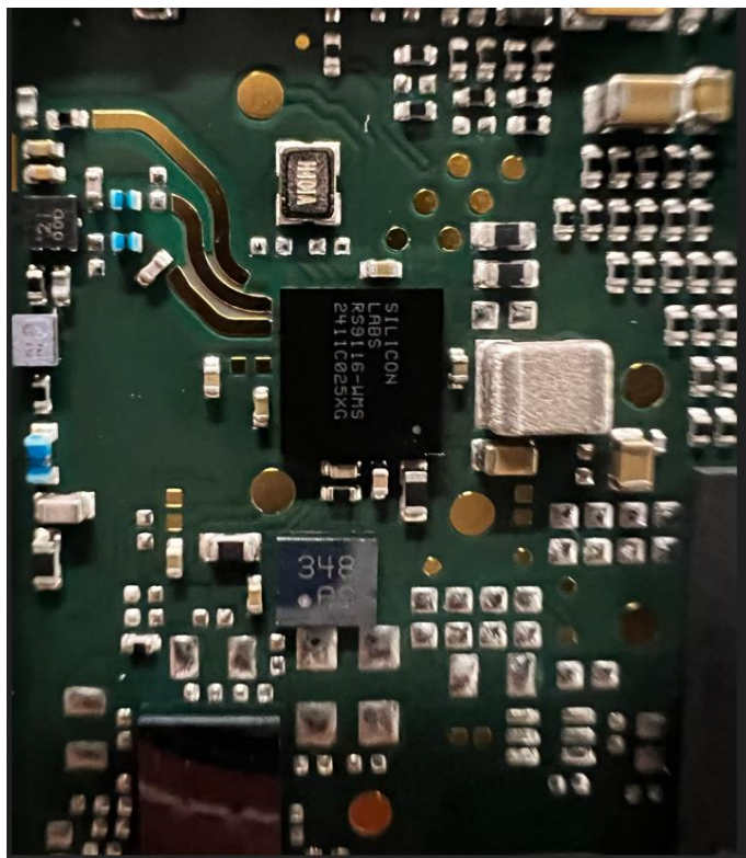
Main Board – Close up of RF Chip
