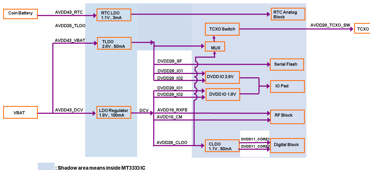
Figure 5-4: Power supply connection (low cost)
