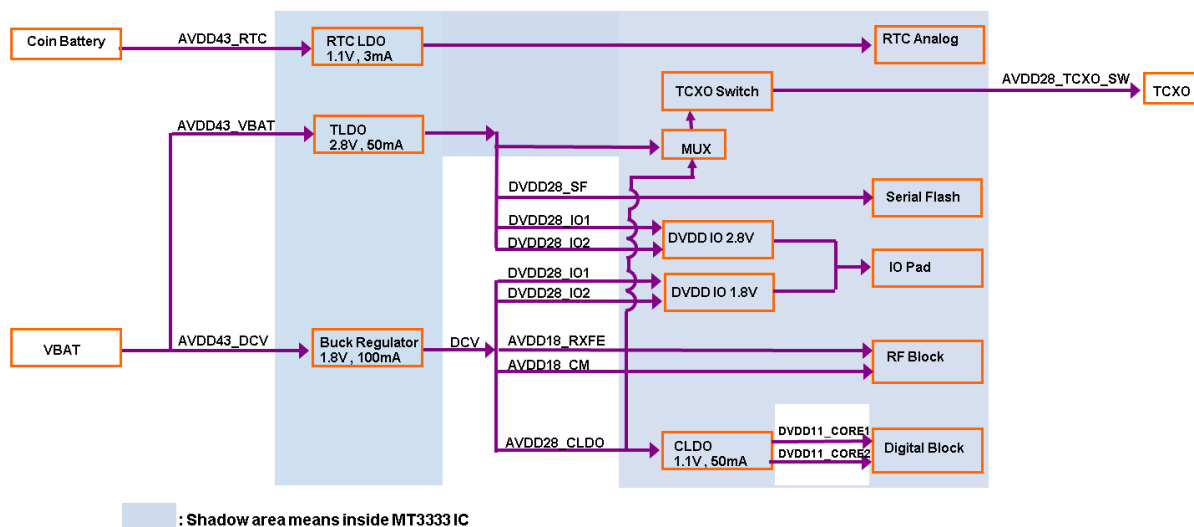
Figure 5-3: Power supply connection (low power)
