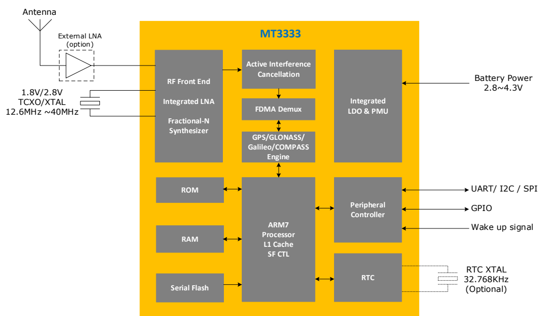
Figure 3-1: MT3333 system block diagram
