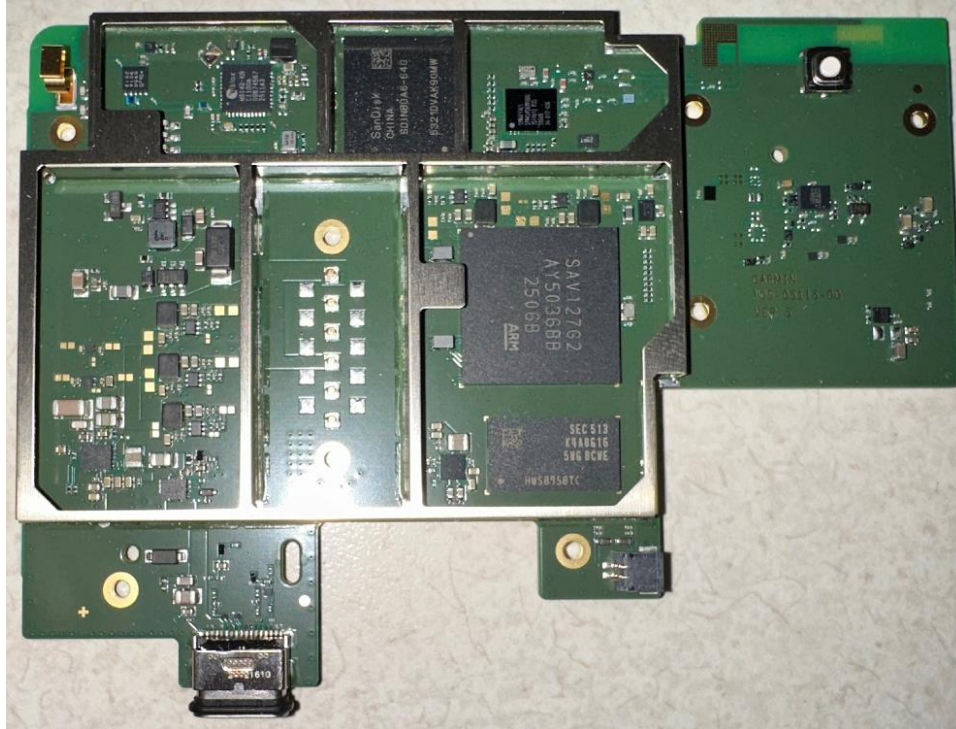
Photograph 07-3: Back side view of the main board, shield removed
