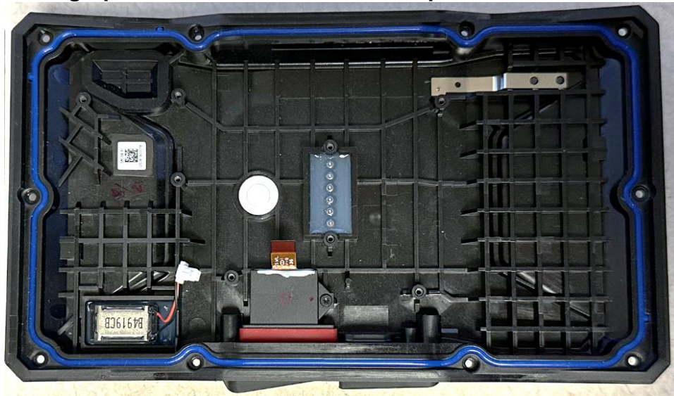
Photograph 07-4: Lower enclosure components
