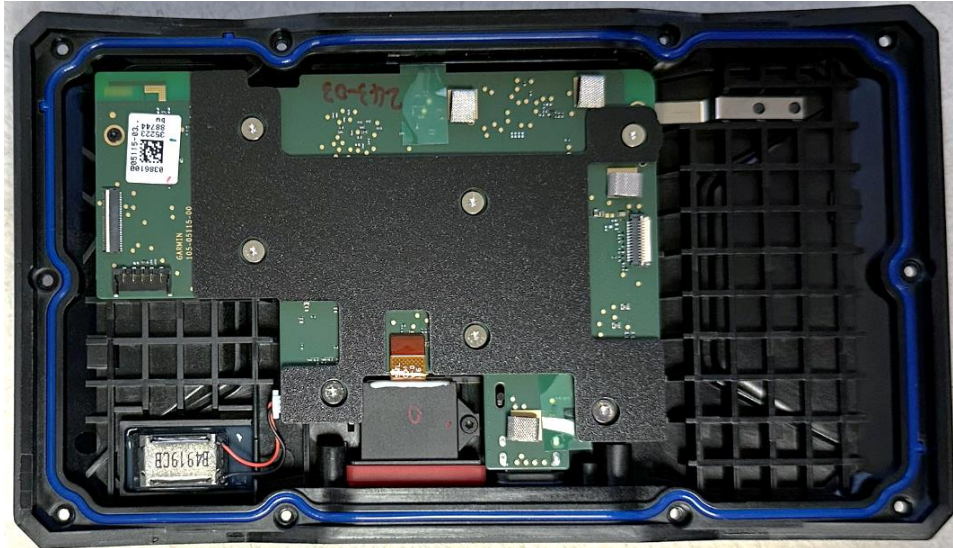
Photograph 07-5: Lower enclosure components, mainboard in place
